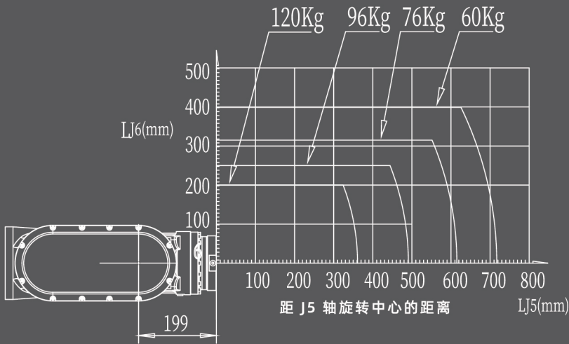
SF120-C2269 Wrist load torque chart
