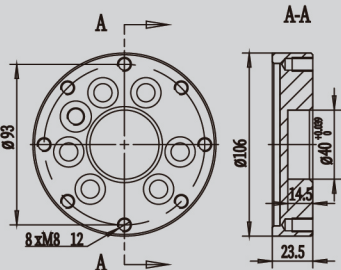
B-Way Diagram (Base Mounting Dimensions)
