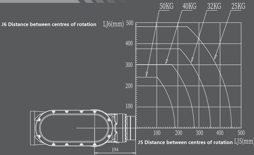
SF50-C2185 Wrist load torque chart
