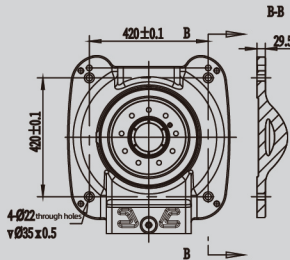
B-Way Diagram (Base Mounting Dimensions)
