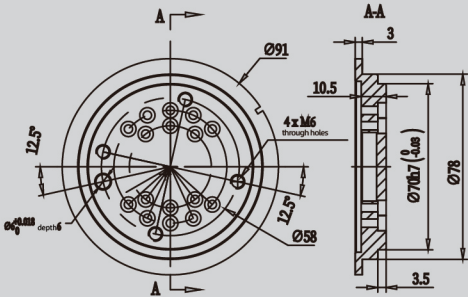
B-Way Diagram (Base Mounting Dimensions)
