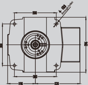
B-Way Diagram (Base Mounting Dimensions)
