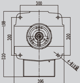
B-Way Diagram (Base Mounting Dimensions)
