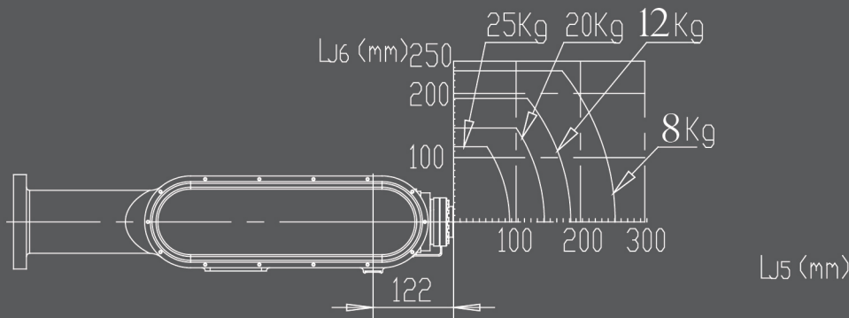
SF25-C1830 Wrist load torque chart
