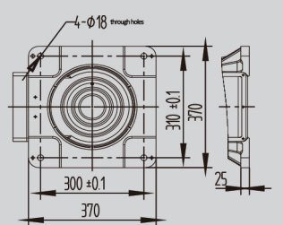
B-Way Diagram (Base Mounting Dimensions)
