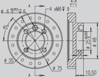
A-Way Diagram (End Flange Mounting Dimensions)
