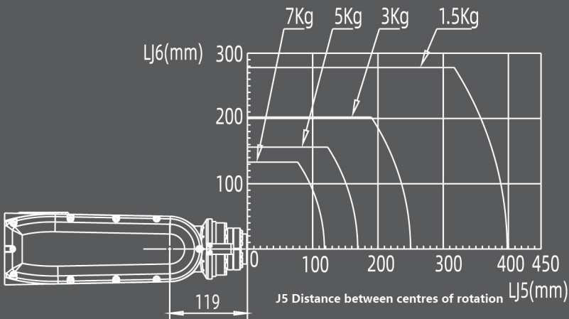
SF7-K759 Wrist load torque chart
